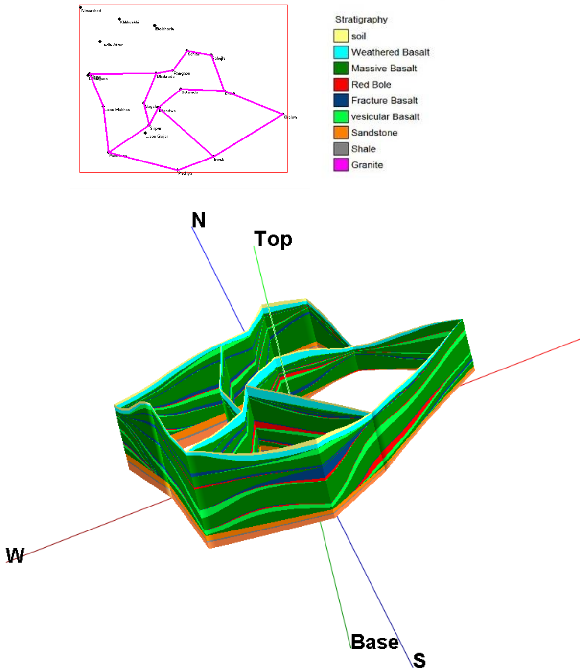
Fig 13: Fence Diagram, Khandwa District, Madhya Pradesh
